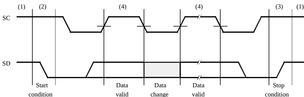
Figure 49. I²C bus protocol 1
