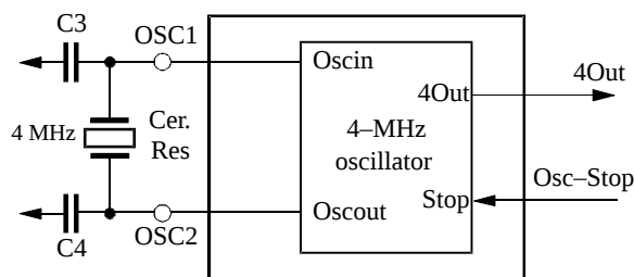
Figure 19. Ceramic resonator
