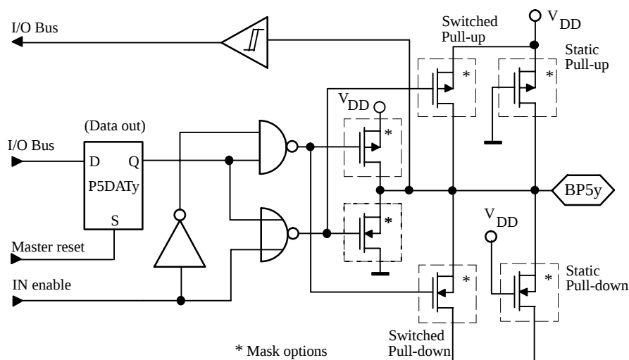
Figure 23. Bidirectional Port 5
