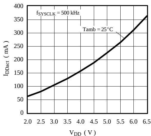
Figure 66. Active supply current vs. V_{DD}
