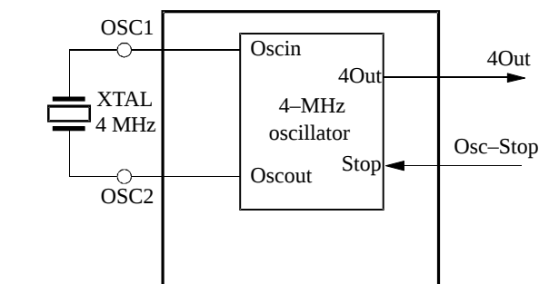
Figure 18. 4-MHz crystal oscillator
