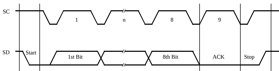
Figure 50. I²C bus protocol 2
