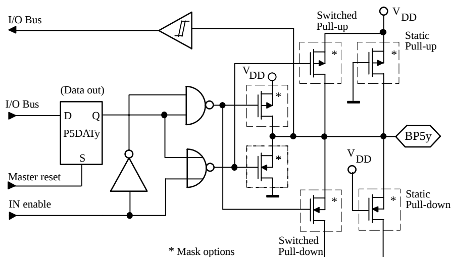
Figure 23. Bidirectional Port 5
