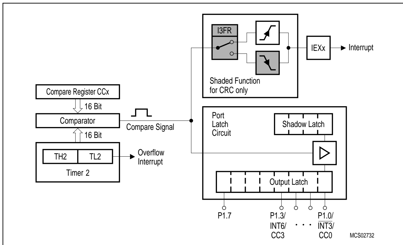
Figure 6-26 Timer 2 with Registers CCx in Compare Mode 1
