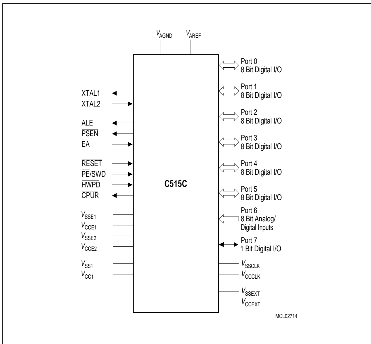
Figure 1-2 Logic Symbol
