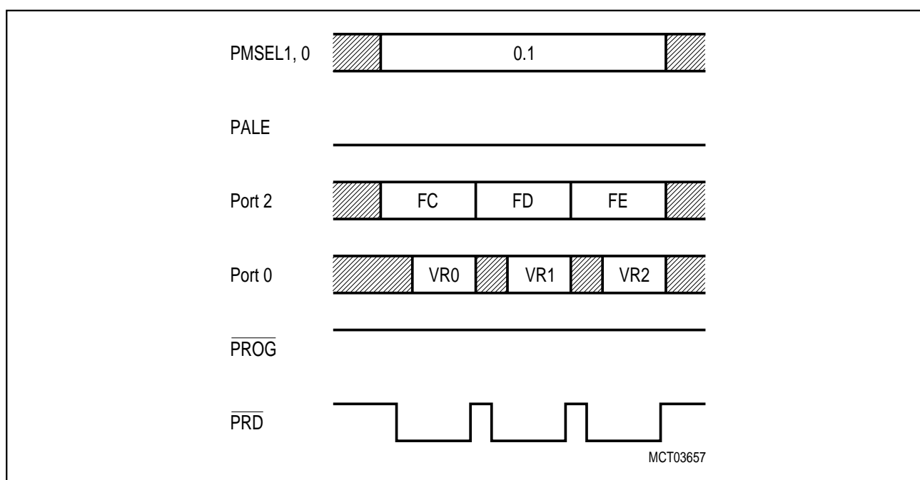
Figure 10-7 Read Version Byte(s) Waveform
