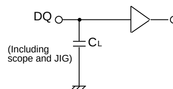
Fig.1 Output load
