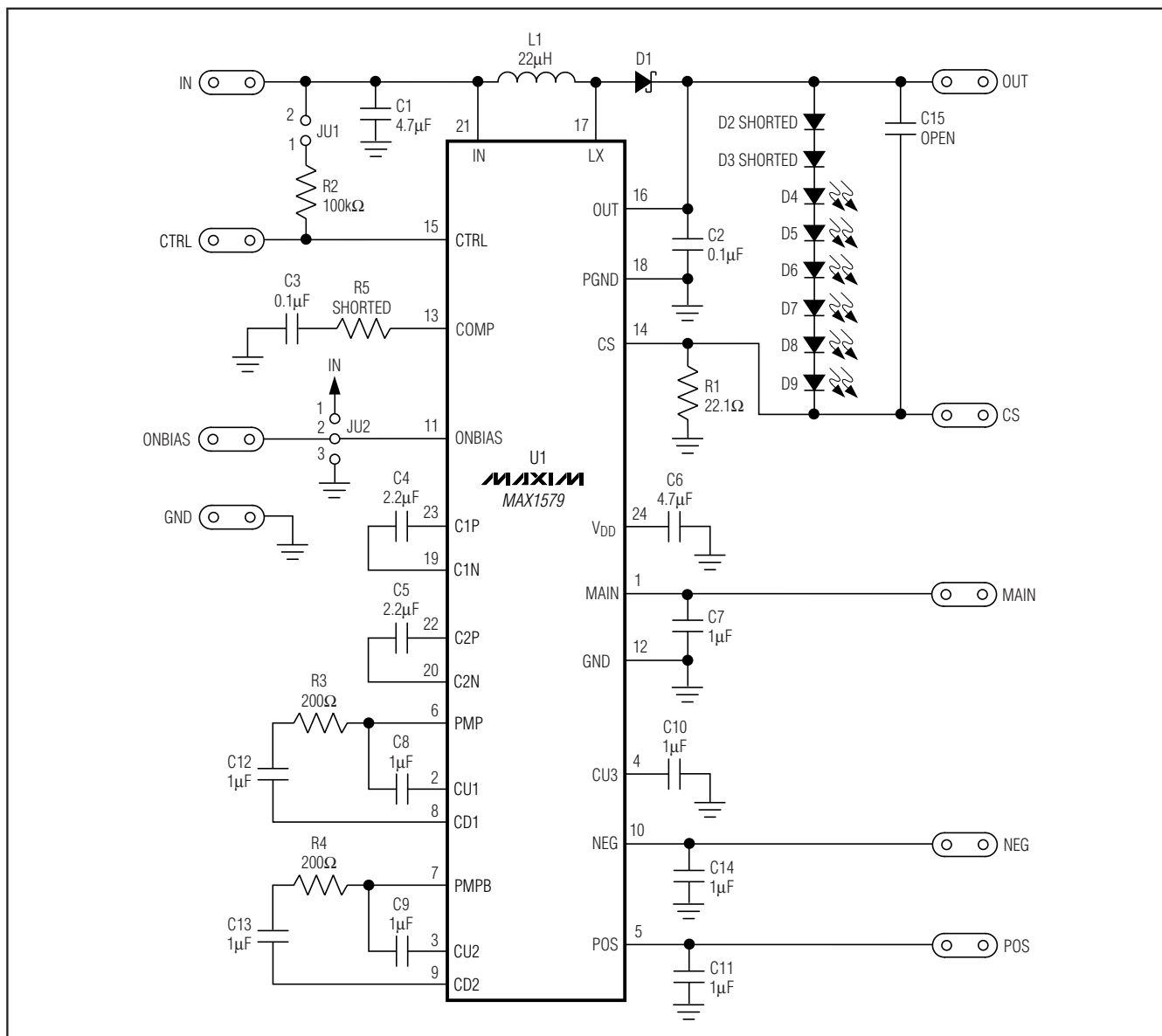
Figure 1. MAX1579 EV Kit Schematic
