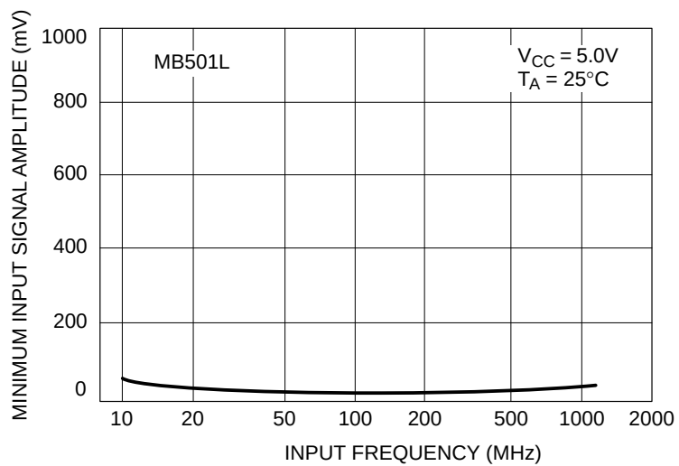
Figure 3. Input Signal Amplitude vs. Input Frequency
