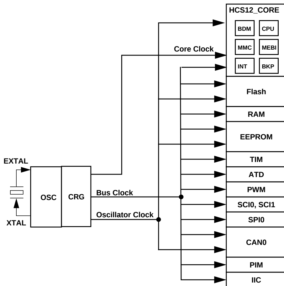
Figure 3-1 Clock Connections
