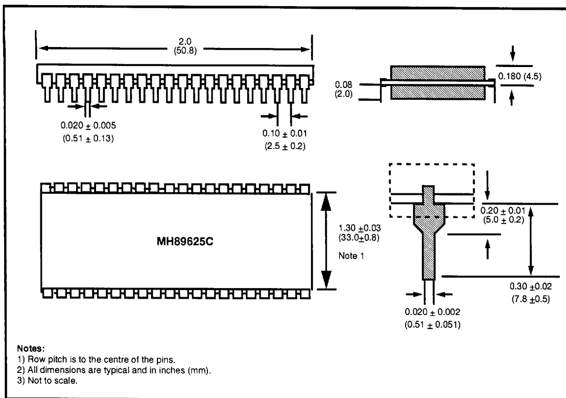
Figure 6 - Mechanical Data
