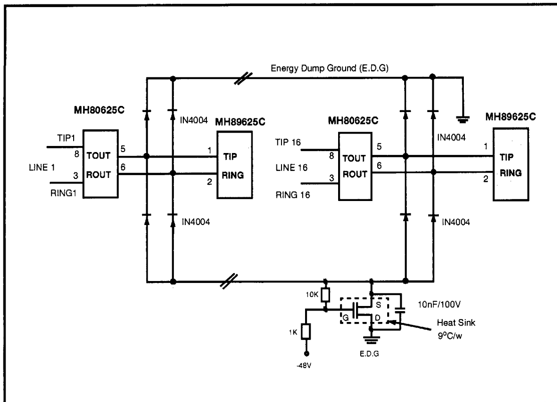
Figure 4 - 16 Lines Circuit Configuration
