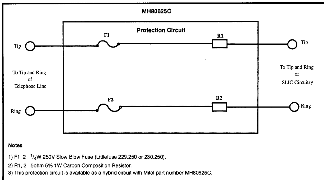
Figure 5 - Solid State External Protection Application Circuit
