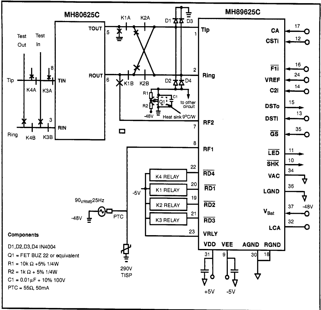
Figure 3 - Typical Line Card Application
