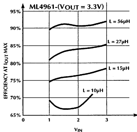
Figure 5. Typical Efficiency as a Function of VIN.
