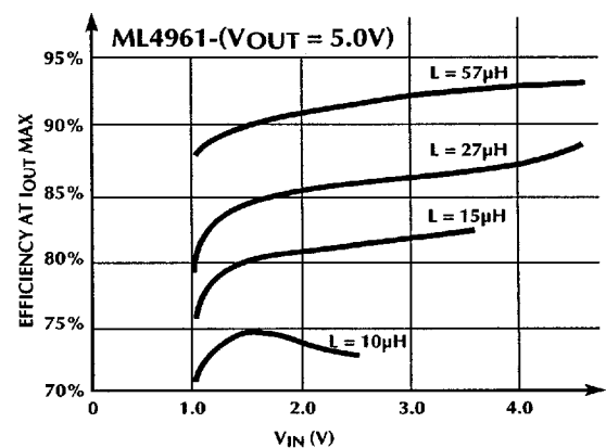
Figure 5. Typical Efficiency as a Function of VIN.
