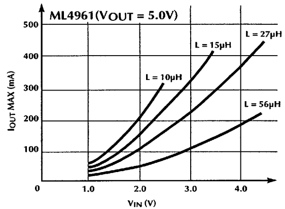
Figure 4. Output Current vs. Input Voltage.
