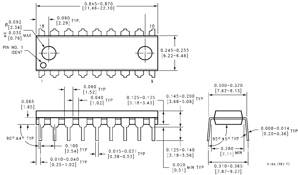
18-Lead Plastic Dual-In-Line Package (PDIP), JEDEC MS-001, 0.300" Wide Package Number N18A
