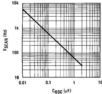
Typical F_{SCAN} vs C_{OSC}
