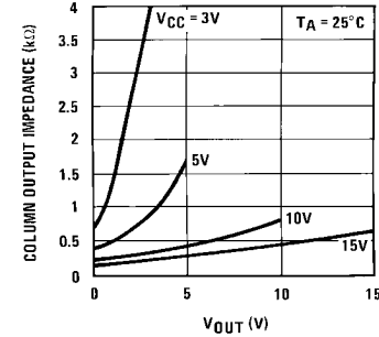
Typical R_{on} vs V_{OUT} at Any X Output
