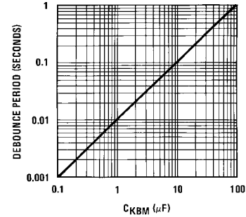
Typical Debounce Period vs C_{KBM}
