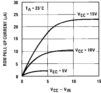
Typical I_{rp} vs V_{IN} at Any Y Input
