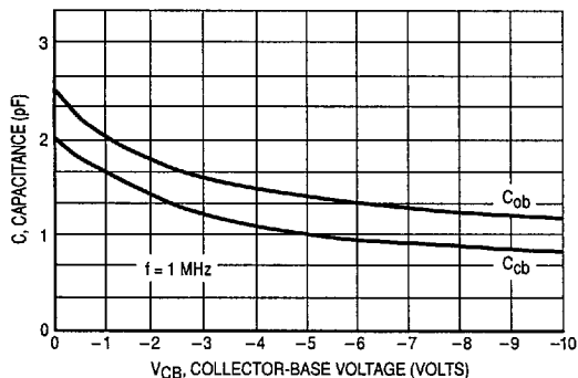
Figure 1. Junction Capacitance versus Voltage
