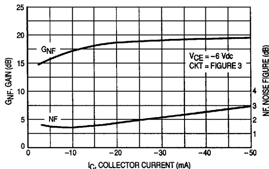
Figure 11. Tuned Circuit — Frequency 500 MHz
