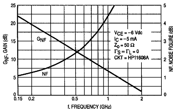
Figure 9. 50 Ohm System
