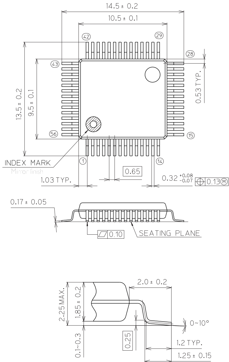
56-Pin Plastic QFP
