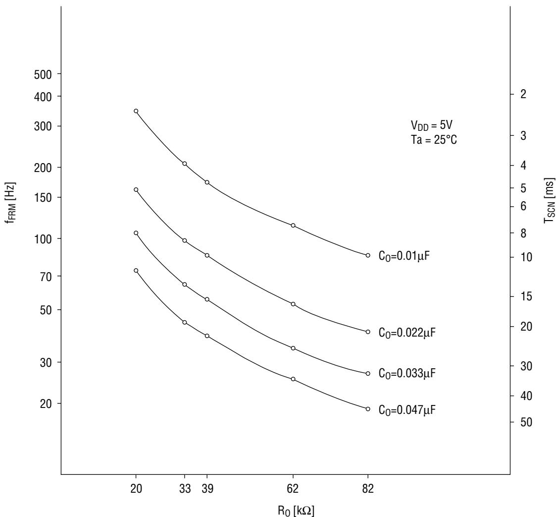
f_{FRM} and T_{SCN} vs. R_0 vs. C_0
