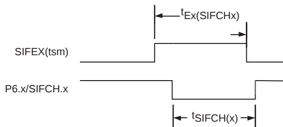
Figure 18. P6.x/SIFCHx timing, SIFCHx function selected
