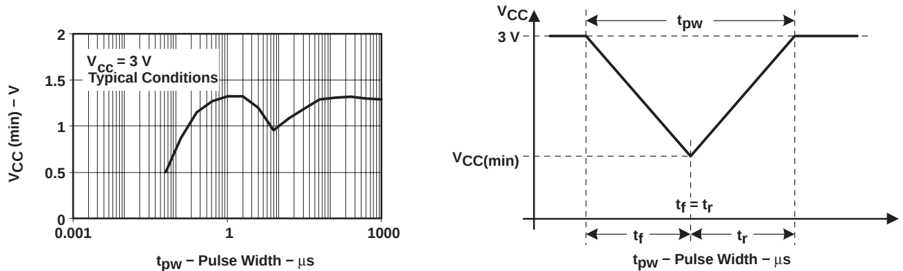
Figure 12. V_{CC(min)} Level With a Triangle Voltage Drop to Generate a POR/Brownout Signal SVS (supply voltage supervisor/monitor) (See Notes 1 and 2)
