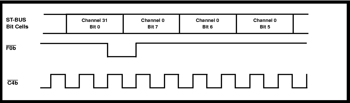
Figure 21 - ST-BUS Functional Timing Diagram
