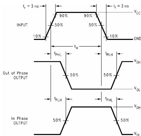
FIGURE 3. AC Waveforms
