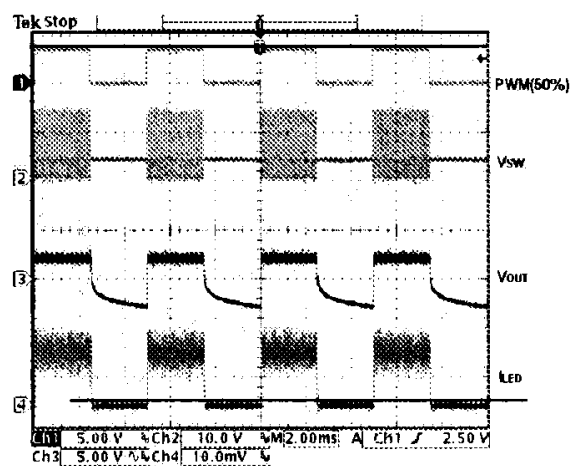
PWM Dimming
