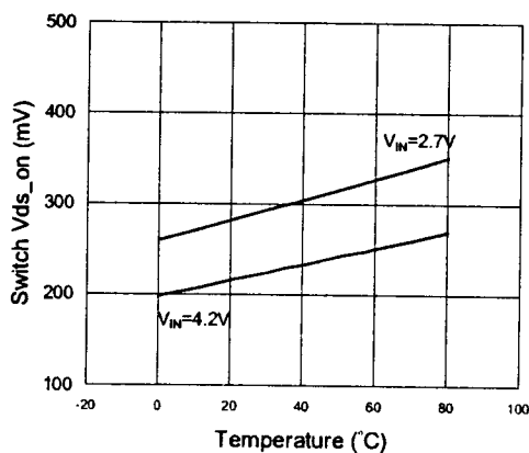
V_{DS(ON)} vs. Temperature
