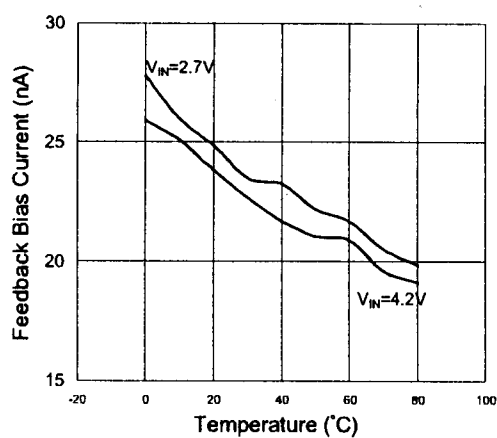
FB Bias Current vs. Temperature
