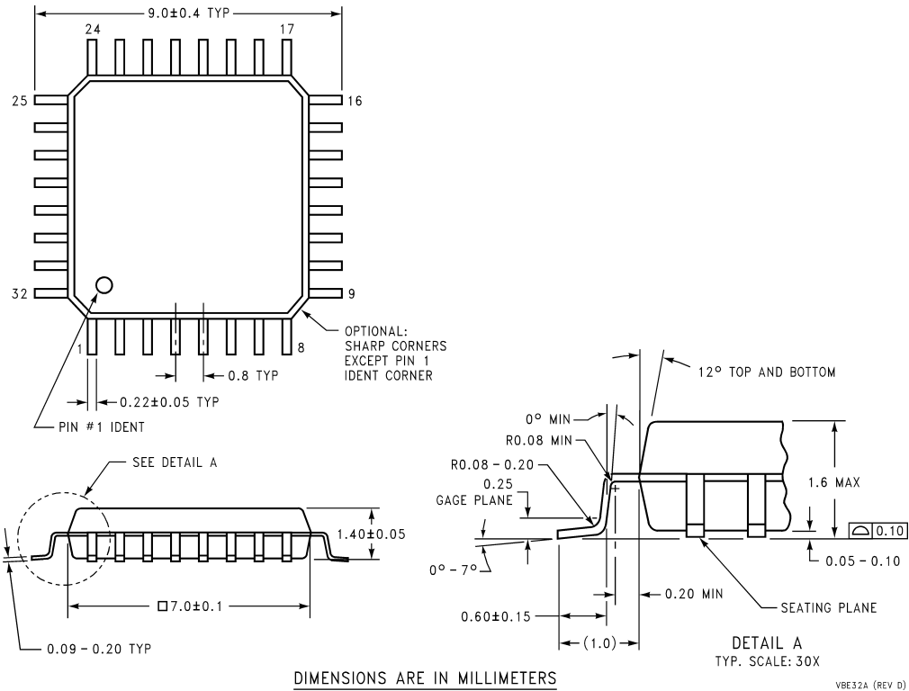
32-Lead TQFP Package Ordering Number ADC10321CIVT NS Package Number VBE32A
