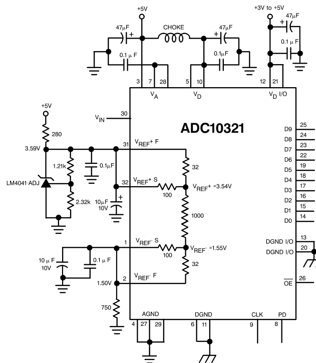
FIGURE 4. Simple, low component current reference biasing
