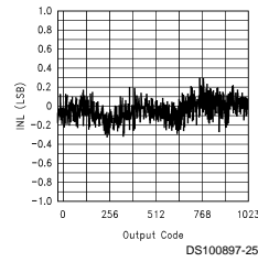
Typical INL
