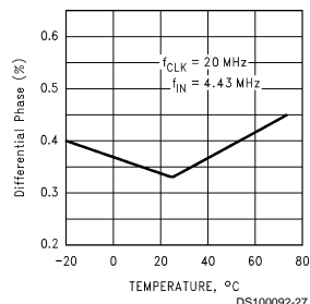
Differential Phase vs Temperature
