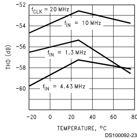
THD vs Temp
