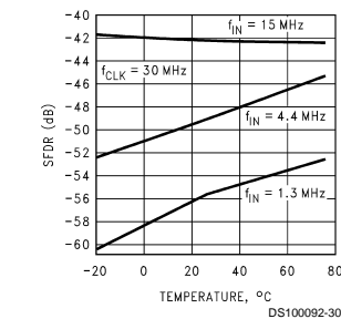
SFDR vs Temp and f_{IN}
