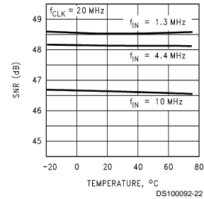
SNR vs Temp at f_{CLK}
