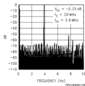
Spectral Response at f_{CLK} = 20 MSPS
