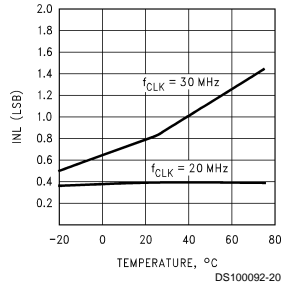
INL vs Temp at f_{CLK}
