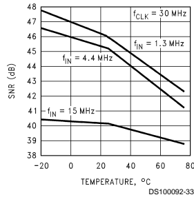
SNR vs Temp at f_{CLK}
