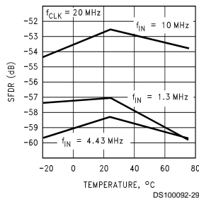
SFDR vs Temp and f_{IN}
