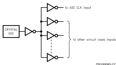
FIGURE 7. Isolating the ADC clock from Digital Circuitry.
