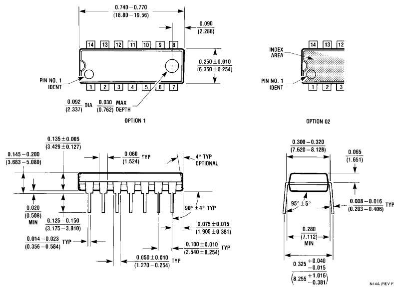
Order Number DS14C89AN NS Package Number N14A
