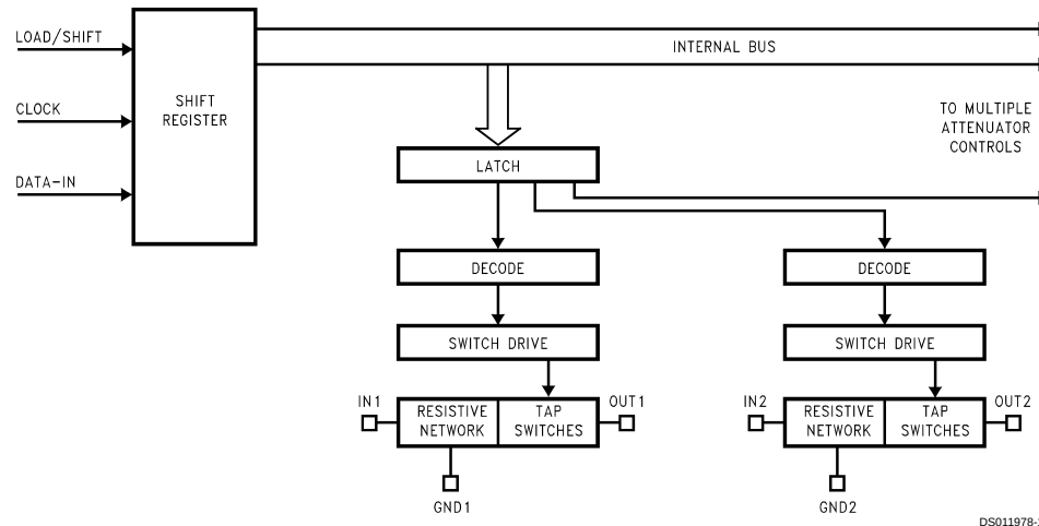
FIGURE 9. μPot System Architecture
