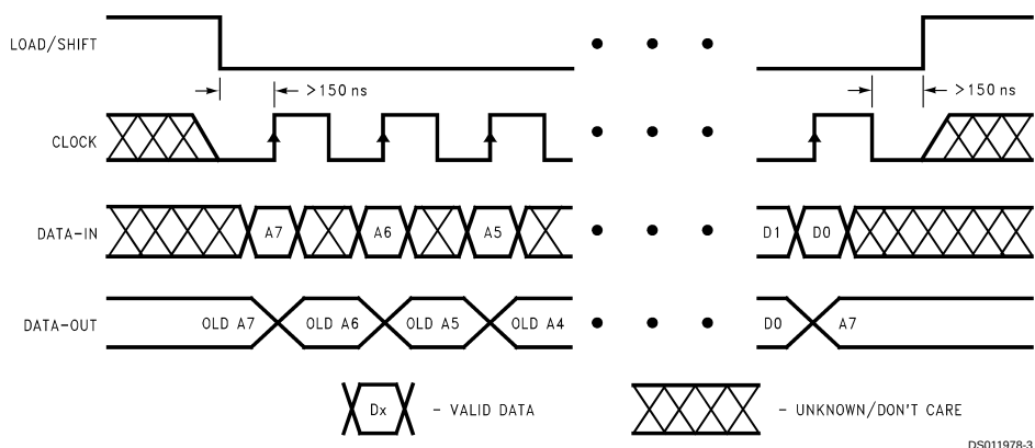
FIGURE 2. Timing Diagram
