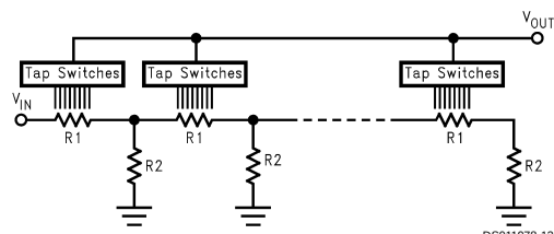
FIGURE 8. μPot Ladder Architecture
