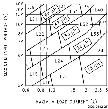
FIGURE 4. LM2599-3.3
