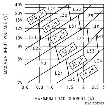
FIGURE 5. LM2599-5.0
