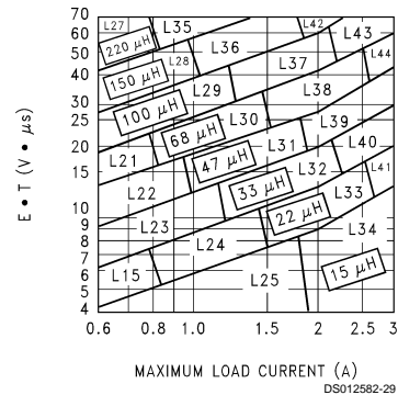
FIGURE 7. LM2599-ADJ
