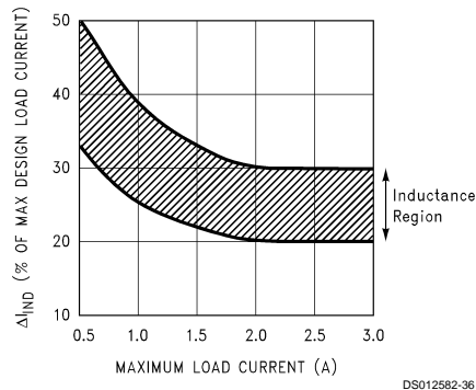
FIGURE 18. ( \Delta_{IND} ) Peak-to-Peak Inductor Ripple Current (as a Percentage of the Load Current) vs Load Current
