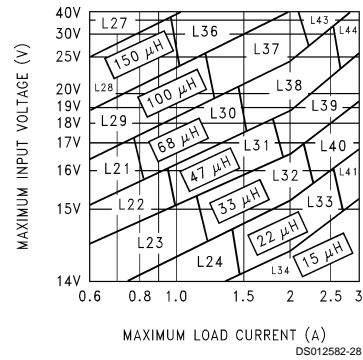
FIGURE 6. LM2599-12
