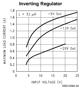
FIGURE 27. Maximum Load Current for Inverting Regulator Circuit
