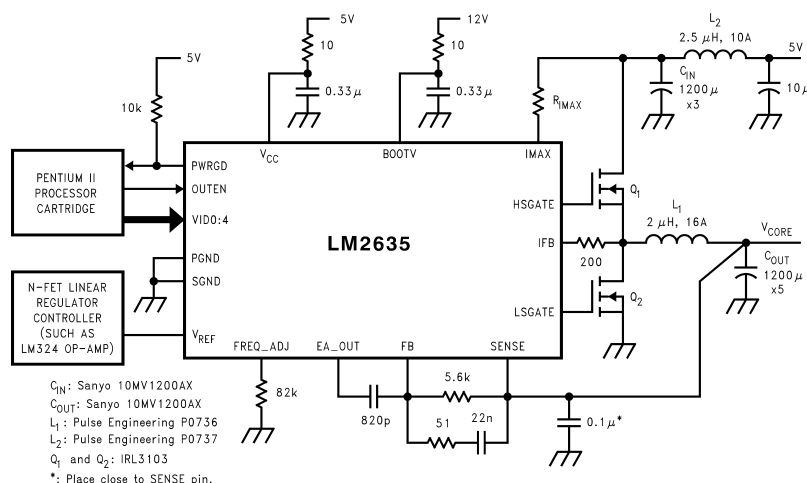
FIGURE 1. 5V to 1.8V–3.5V, 14A Power Supply
