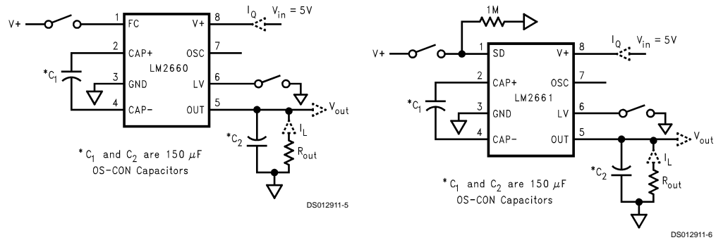
FIGURE 1. LM2660 and LM2661 Test Circuits
