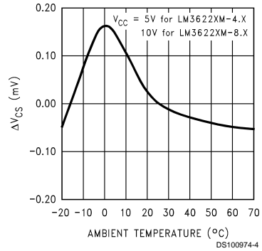
Current Sense Voltage Regulation Vs Temperature
