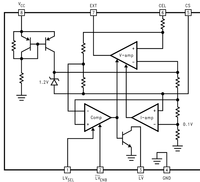
FIGURE 1. LM3622 Simplified Block Diagram
