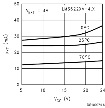
Output Drive Current Vs V_{CC}
