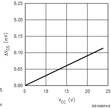
Current Sense Voltage Regulation Vs V_{CC}
