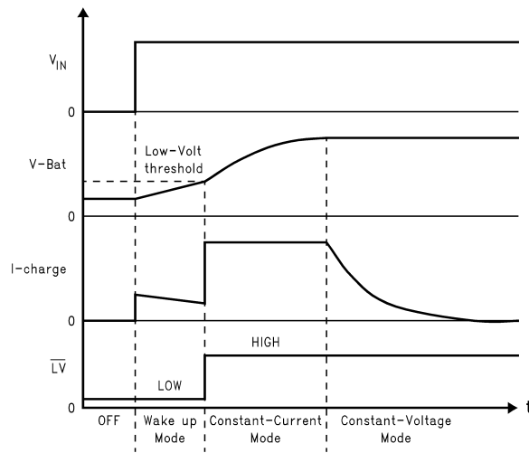
FIGURE 3. Typical Charge Cycle with Low-Voltage Detection Enabled.
