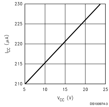
Quiescent Current Vs V_{CC}
