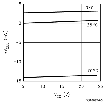
Output Voltage Regulation Vs V_{CC}
