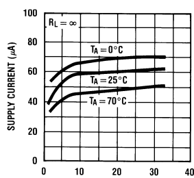
Supply Current
