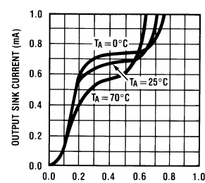
Output Sink Current
