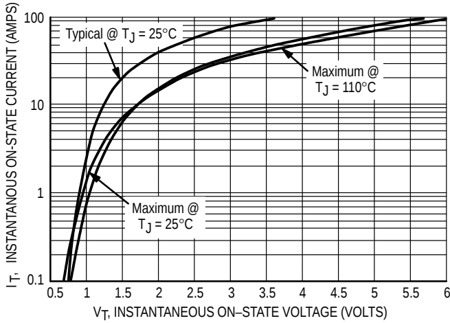
Figure 3.0 On-State Characteristics
