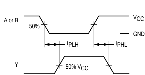
Figure 3. Switching Waveforms
