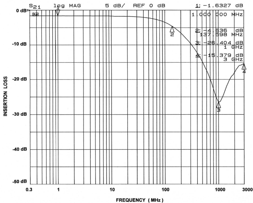
Figure 4. Insertion Loss vs. Frequency Performance Curve, PACUSB-D3(SOT23-6)
