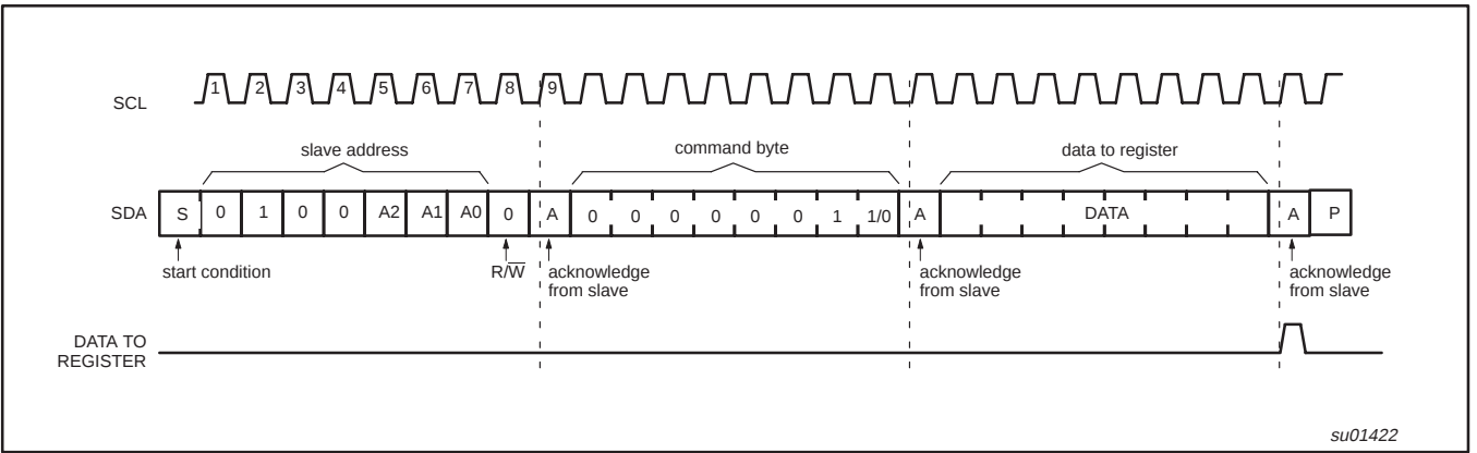
Figure 7. WRITE to configuration or polarity inversion registers
