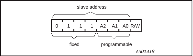
Figure 5. PCA9554A address
