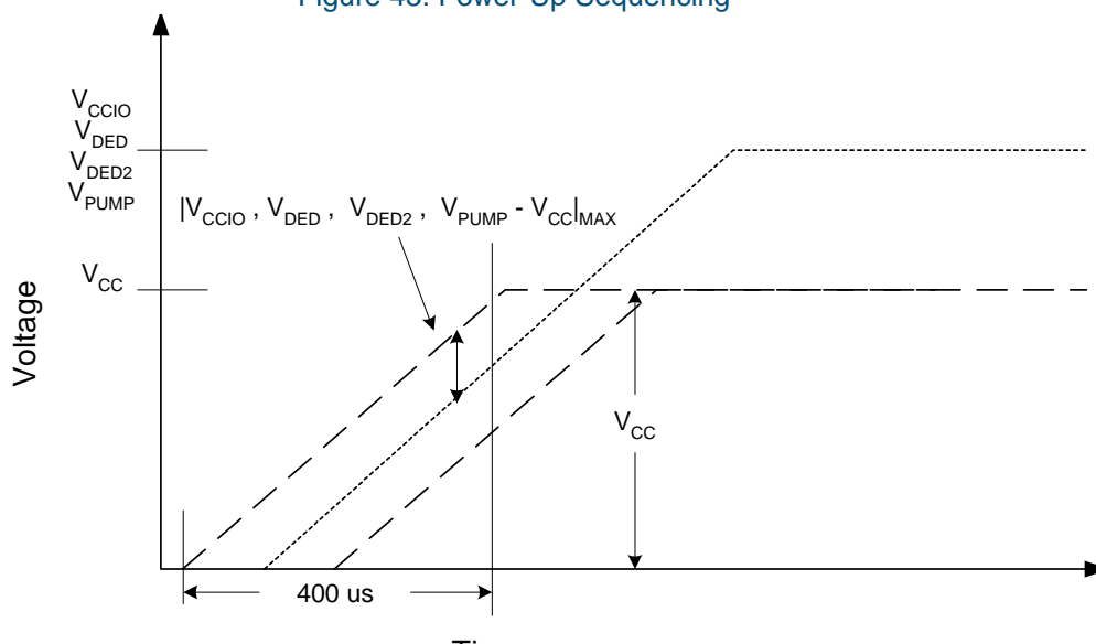
Figure 45: Power-Up Sequencing
