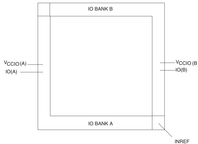
Figure 1: QL5810 and QL5820 I/O Banks with Relevant Pins
