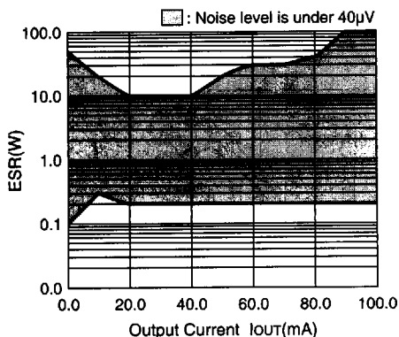
Ceramic Capacitor 4.7 \mu F
