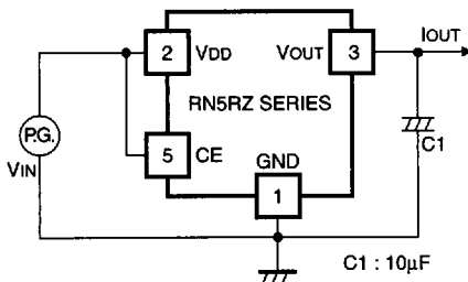
Fig.3 Line Transient Response Test Circuit
