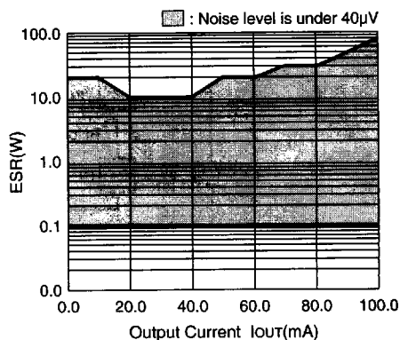
Ceramic Capacitor 10 \mu F
