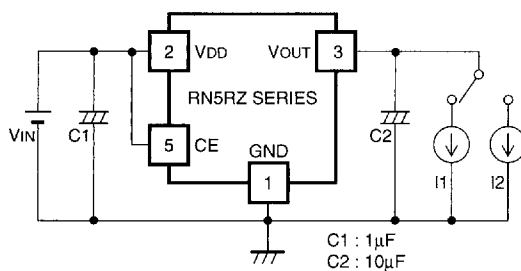
Fig.4 Load Transient Response Test Circuit
