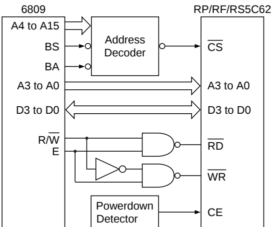
RP/RF/RS5C62 and CPU 6809
