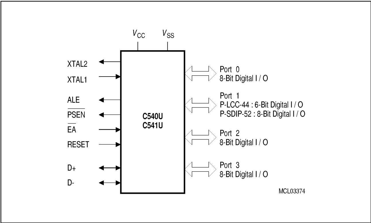
Figure 2 Logic Symbol
