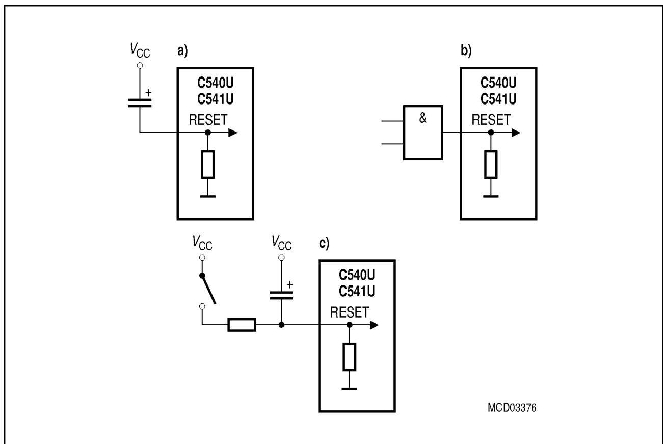
Figure 7 Reset Circuitries
