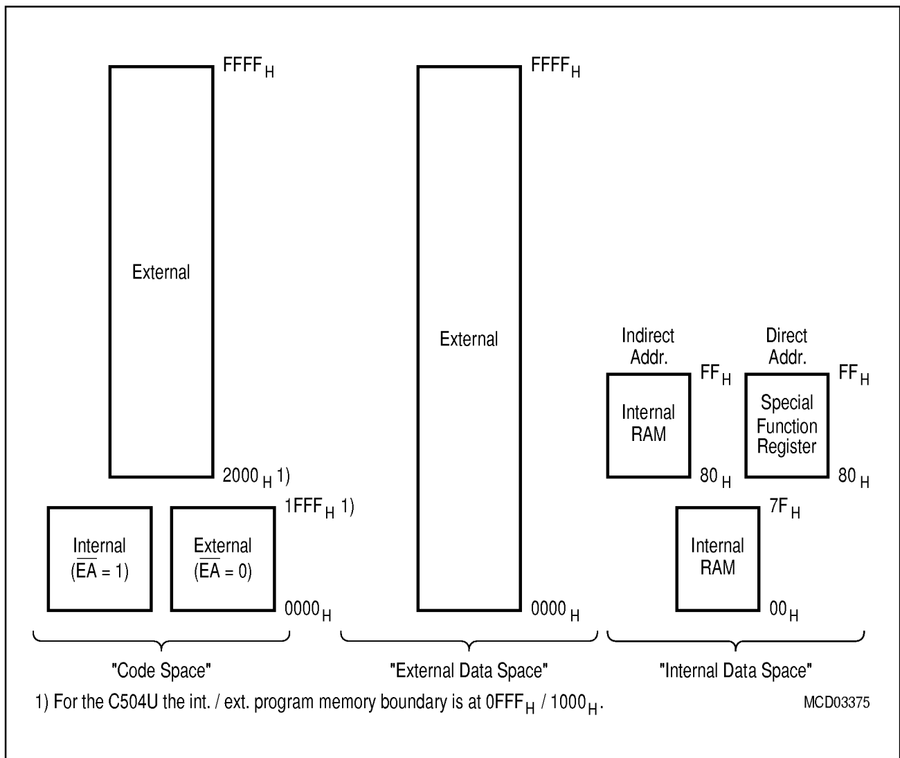
Figure 6 C540U/C541U Memory Map
