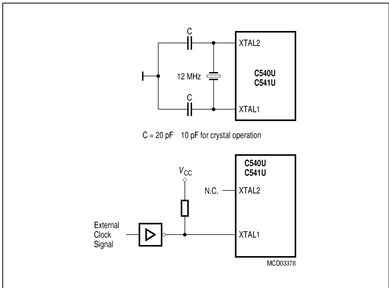
Figure 9 Recommended Oscillator Circuitries
