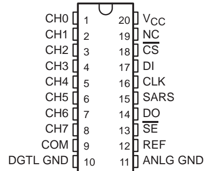
TLC0838 . . . PW, DW, OR N PACKAGE (TOP VIEW)
