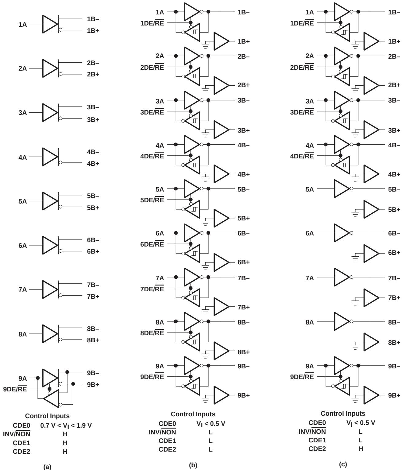
Figure 11. Logic Diagrams
