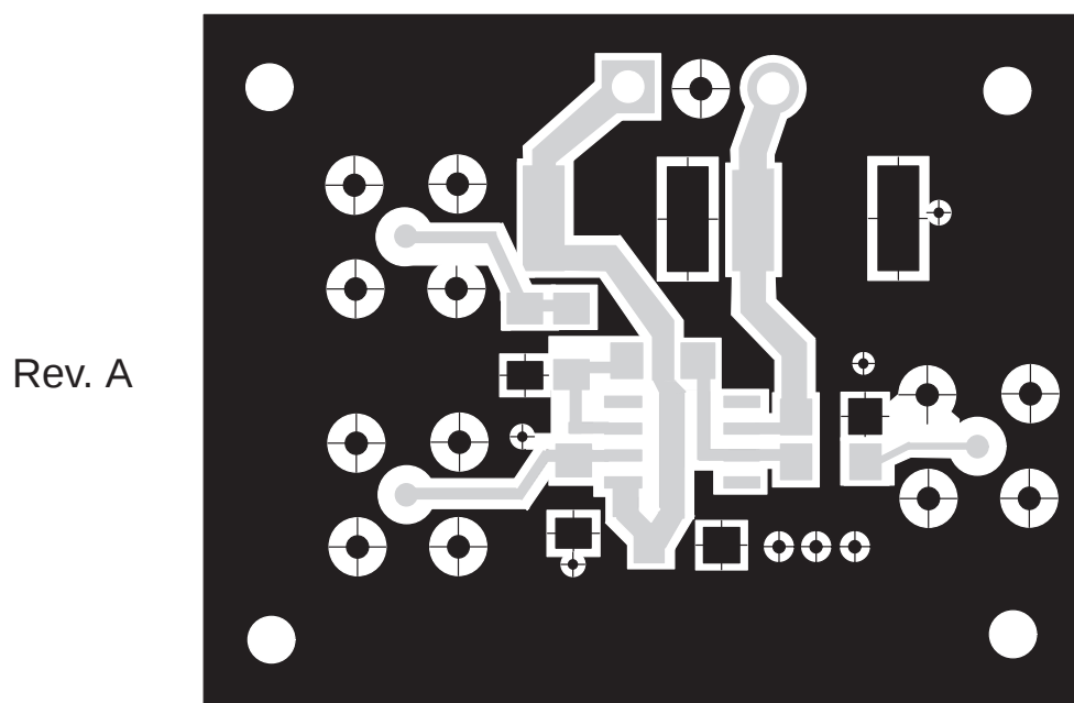
Figure 2–5. THS3001 Rev. A EVM PC Board Layout – Component Side
