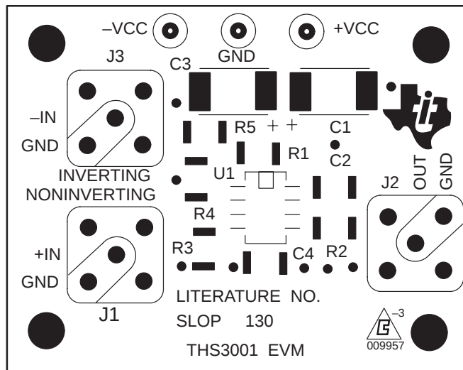
Figure 2–1. THS3001 EVM Component Placement Silkscreen and Solder Pads
