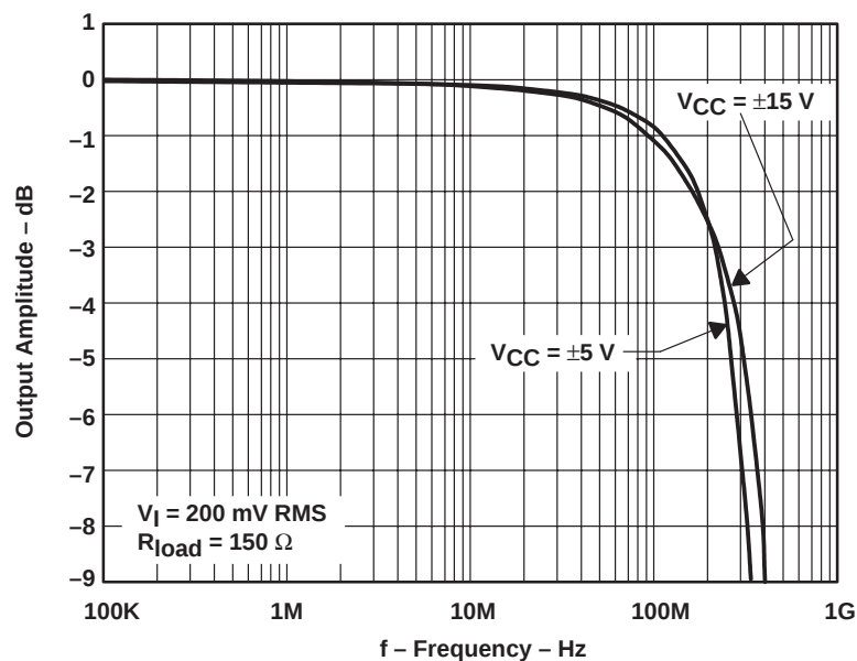
Figure 1–6. THS3001 EVM Frequency Response with Inverting Gain = 1
