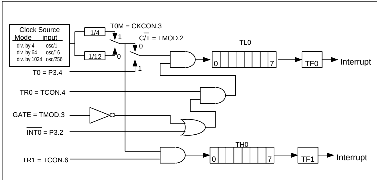
Figure 13. Timer/Counter 0 Mode 3
