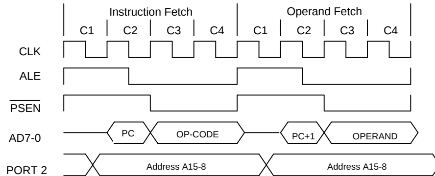
Figure 4. Two Cycle Instruction Timing
