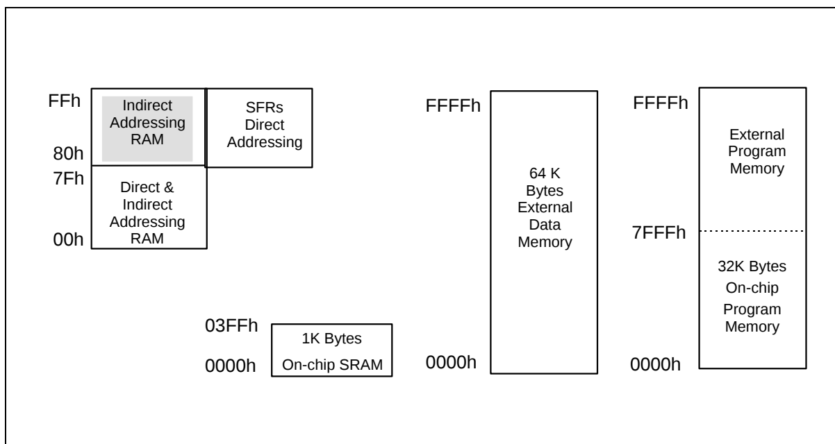
Figure 1. Memory Map
