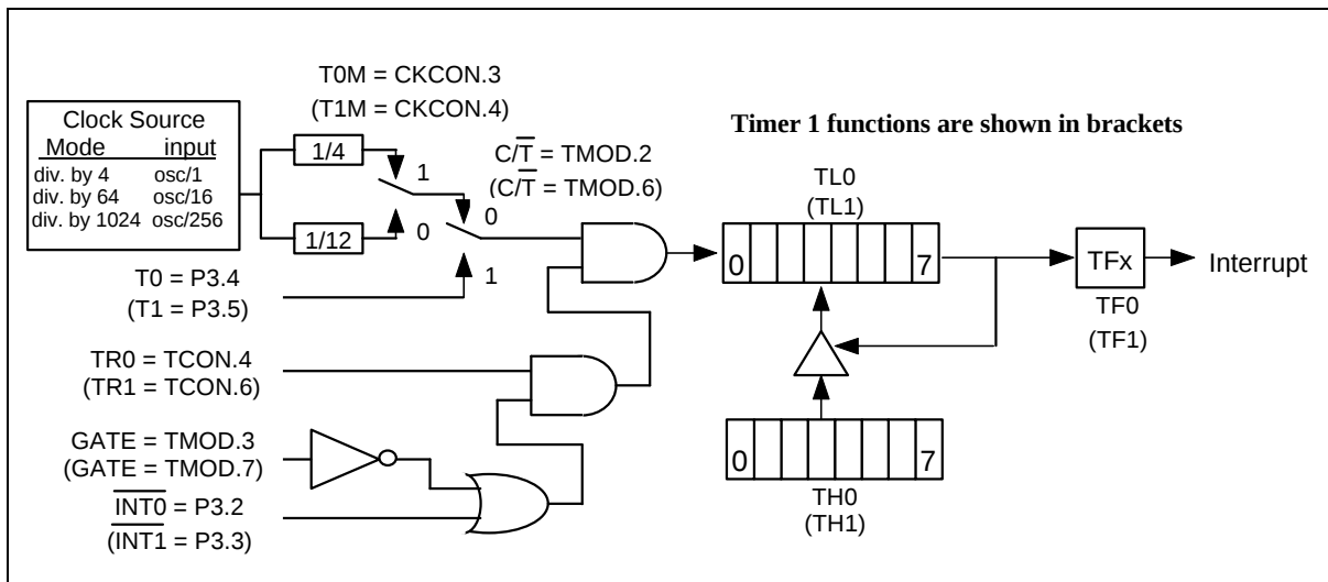
Figure 12. Timer/Counter Mode 2.
