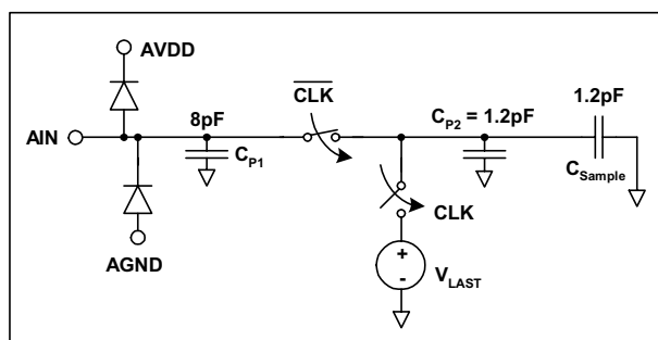
Figure 20 Equivalent Circuit for Analogue Input Pin AIN
