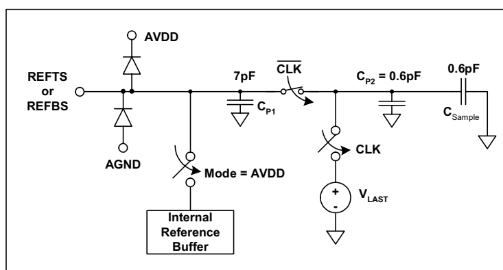
Figure 23 Equivalent Circuit of REFTS and REFBS Sample & Hold Inputs
