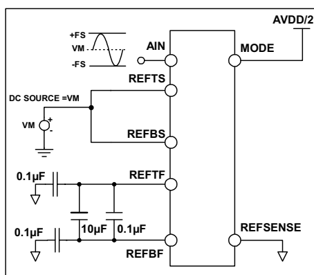
Figure 12 Centre Span Mode, 2V Reference Span
