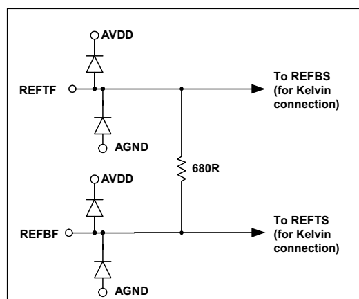
Figure 26 Equivalent Circuit of REFTF and REFBF Inputs
