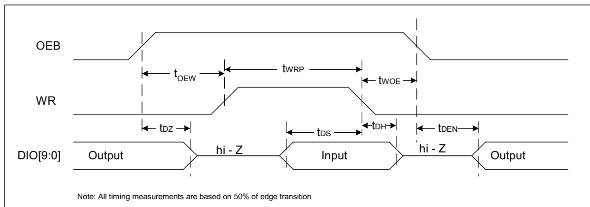
Figure 1 Write Timing
