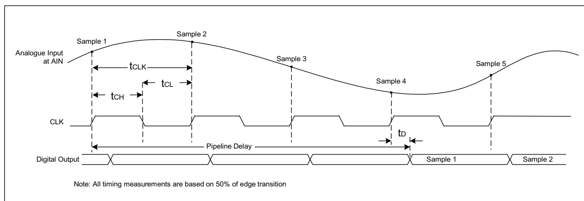
Figure 2 Output Timing
