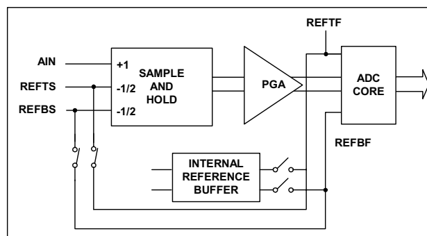
Figure 7 ADC Reference Generation in Full External Mode
