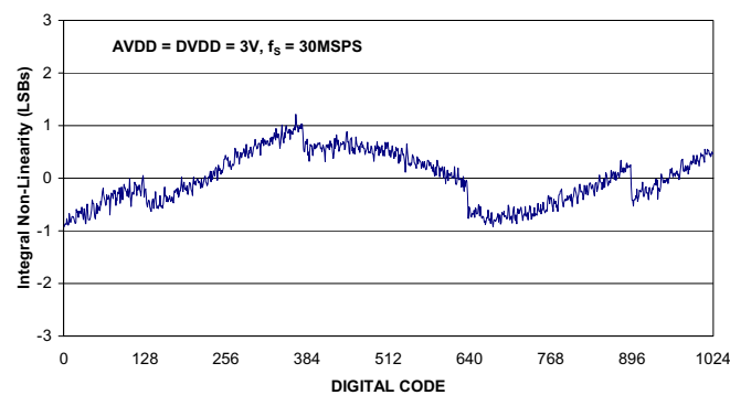
Figure 4 Integral Non-Linearity
