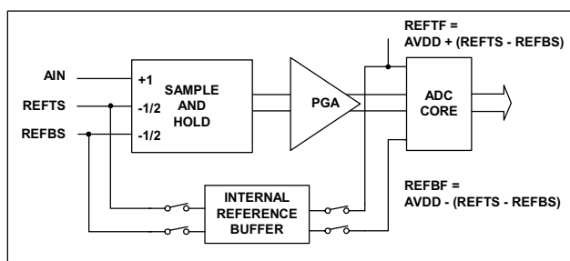
Figure 13 ADC Reference Generation in Top/Bottom Mode
