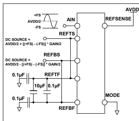
Figure 8 Full External Reference Mode (Reference Generator Disabled)
