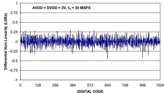
Figure 3 Differential Non-Linearity
