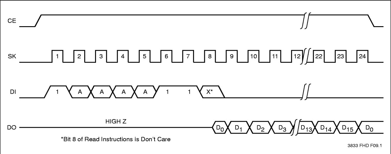
Figure 2. RAM Write
