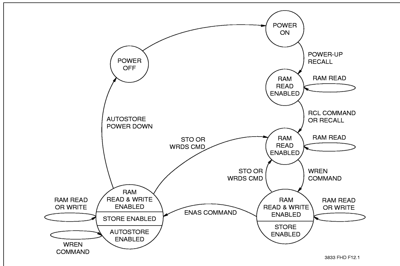
Figure 4. X24C45 State Diagram
