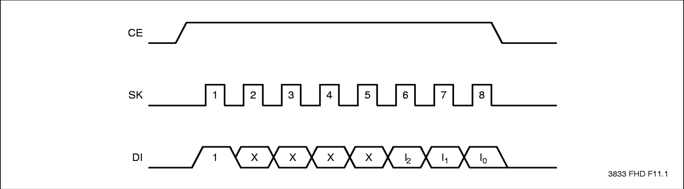
Figure 3. Non-Data Operations
