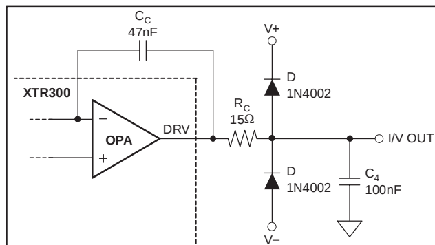
Figure 11. Example for DRV Output Protection
