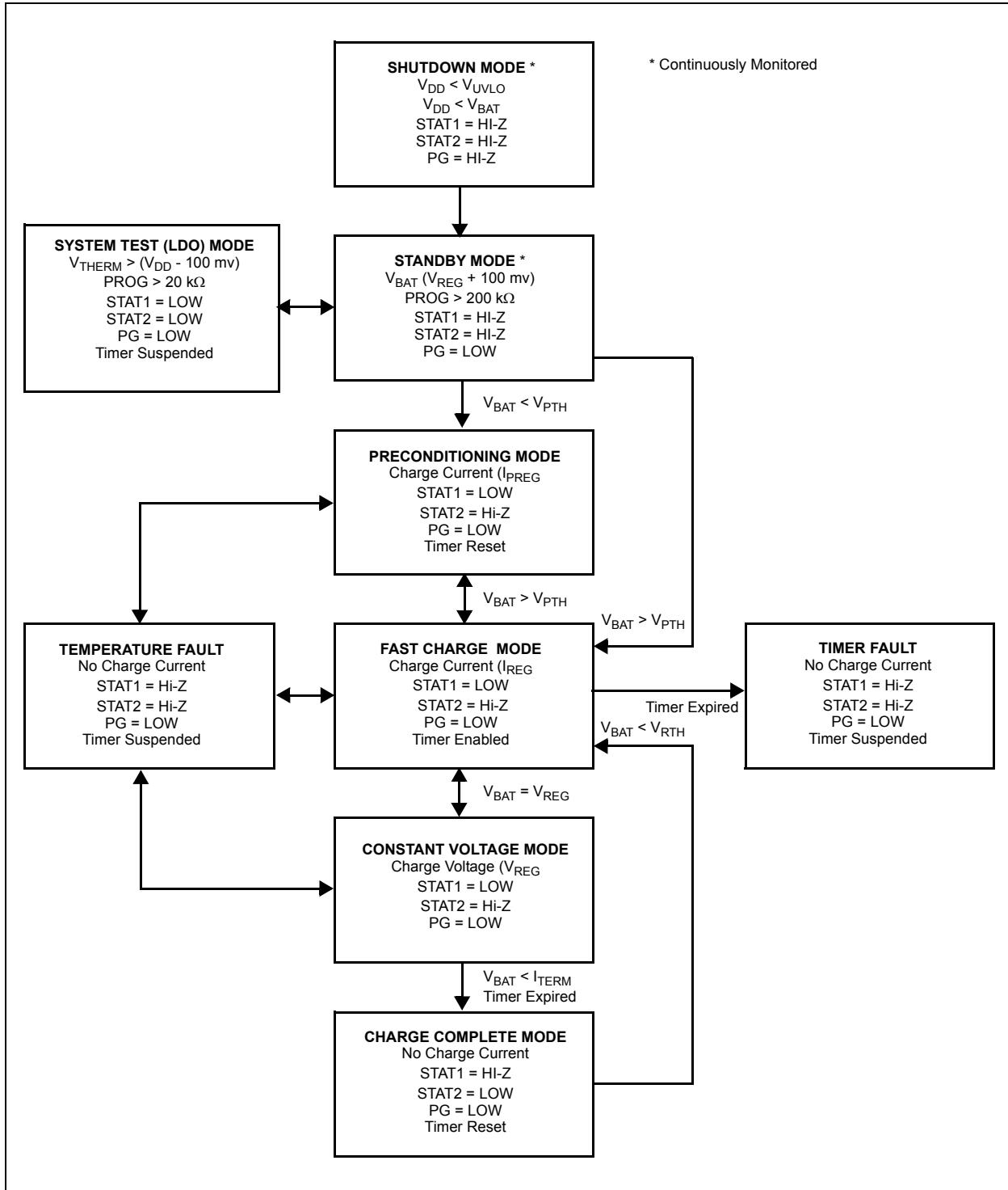
FIGURE 4-1: Flow Chart.
