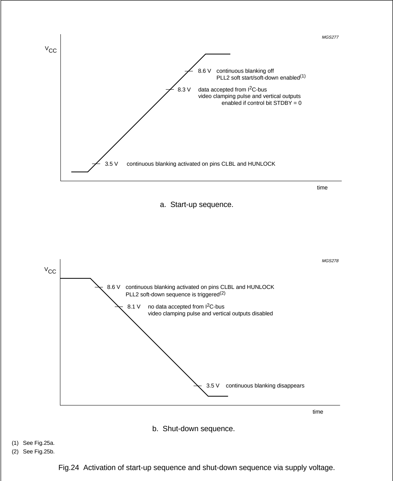
Start-up sequence and shut-down sequence
