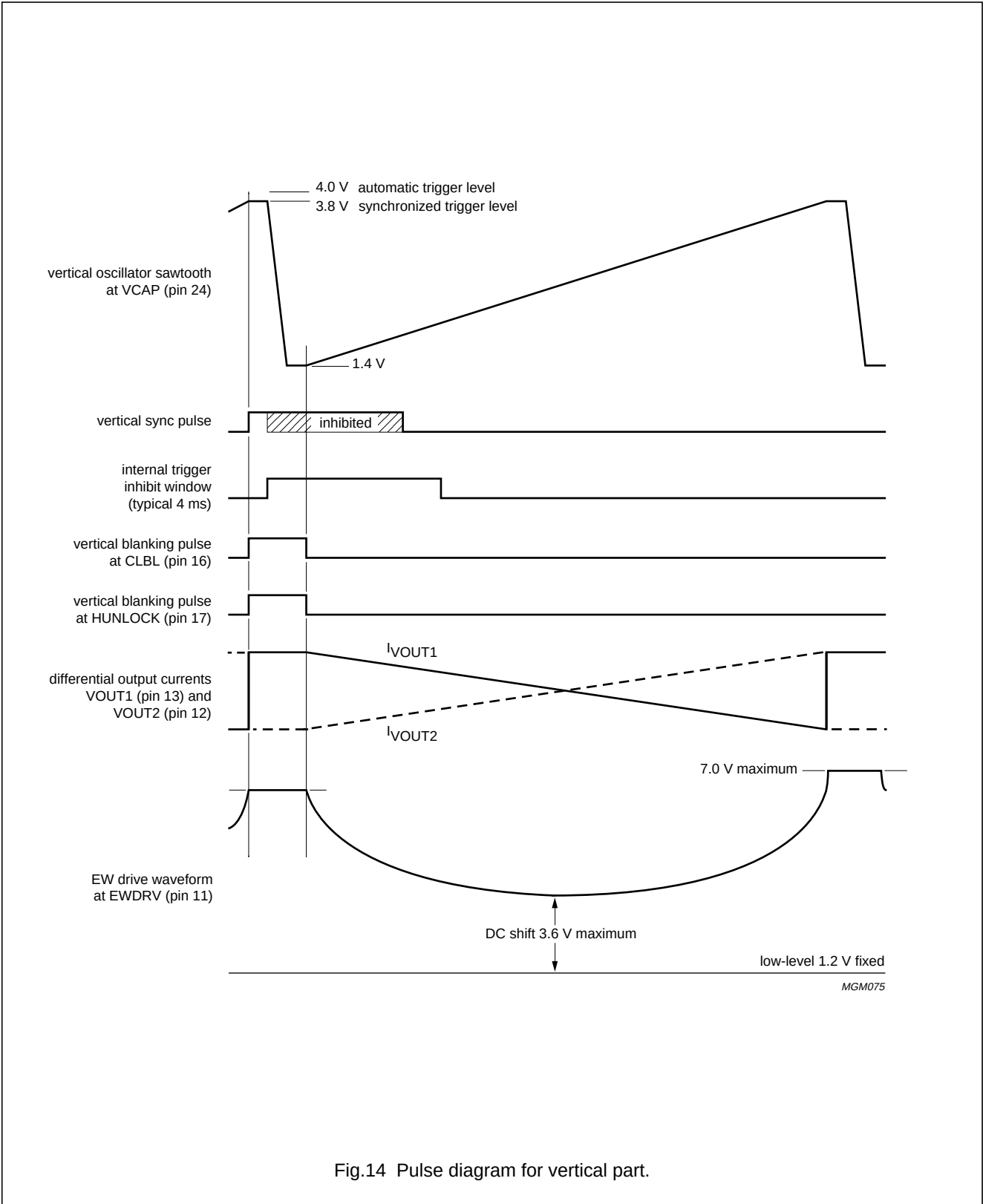
Pulse diagrams
