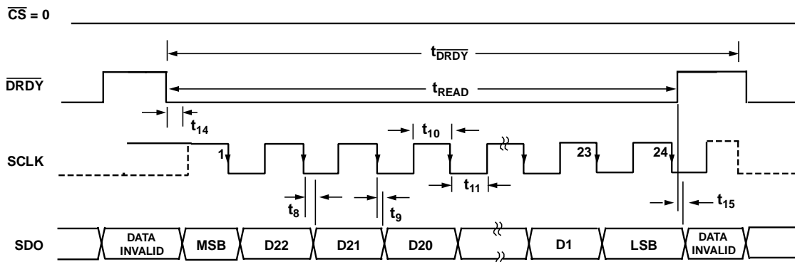
Figure 4. Serial timing diagram, reading data setting \overline{CS} logic low.
