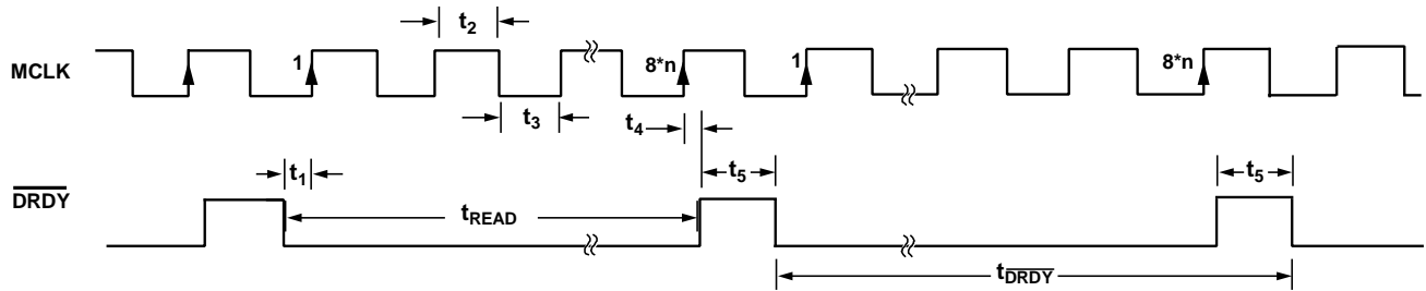
Figure 2. \overline{DRDY} versus MCLK Timing Diagram. For AD7766 n=1 (Decimate by 8), AD7766-1 n=2 (Decimate by 16), AD7766-2 n=4 (Decimate by 32).
