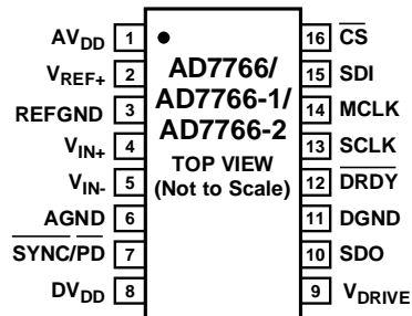
Figure 6.16-16-Lead TSSOP Pin Configuration
