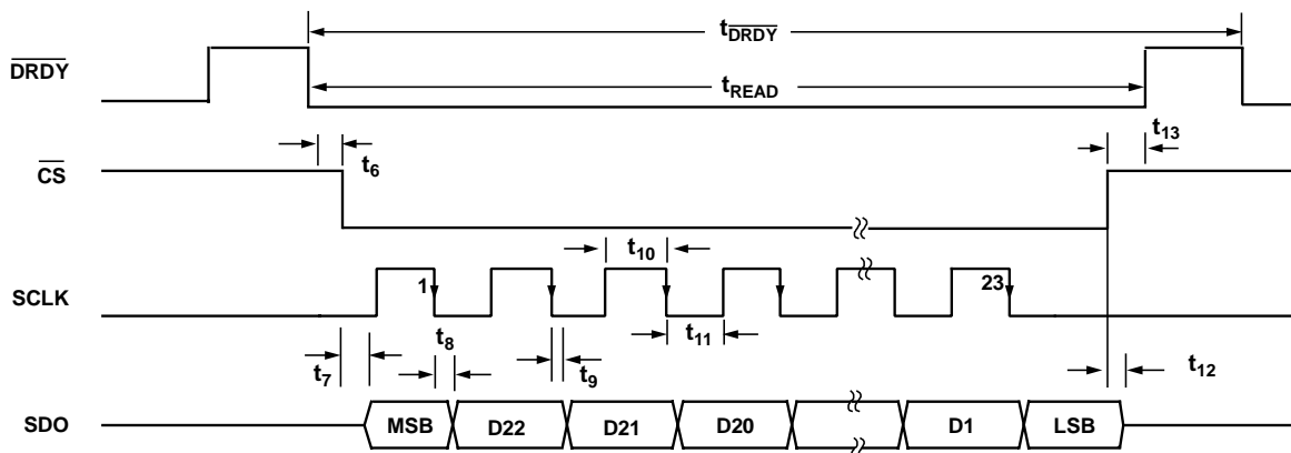
Figure 3. Serial timing diagram, reading data using \overline{CS}
