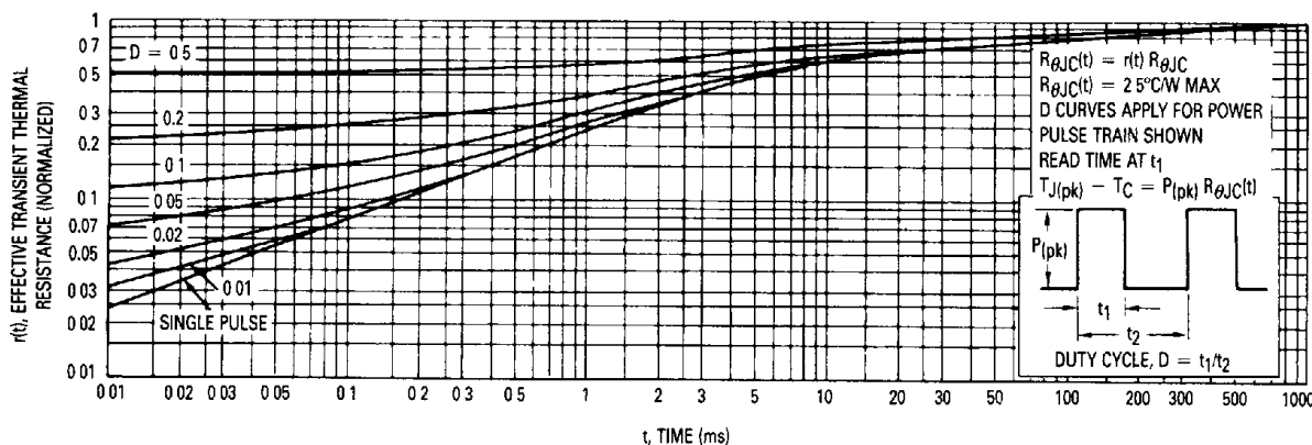
Figure 10. Thermal Response
