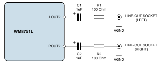
Figure 32 Recommended Circuit for Line Output
