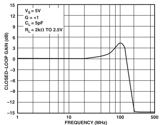
Figure 2. Frequency Response
