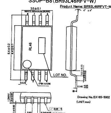
Fig4-(j) PHYSICAL DIMENSION TSSOP-B8 (BR93L46RFVT-W)
