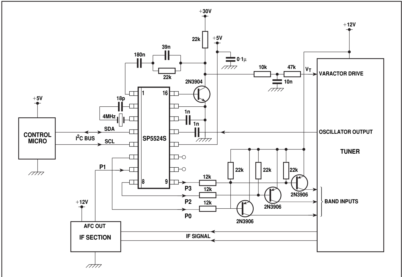
Fig. 4 Typical application
