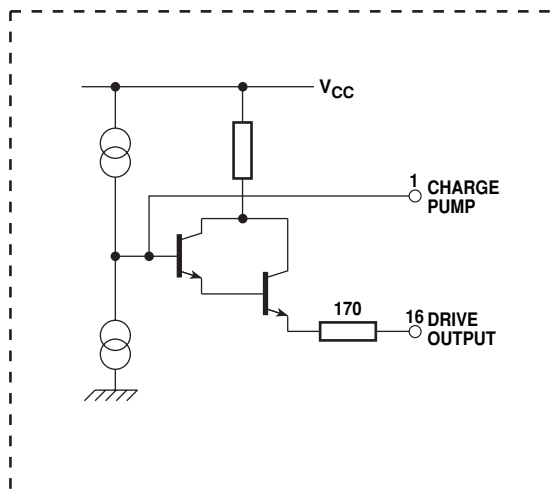
Loop amplifier
